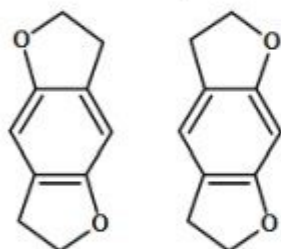
Tetrahydrobenzodifuranyl-
