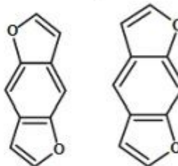
Benzodifuranyl-
