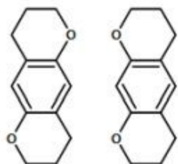
Tetrahydrobenzodipyranyl-
